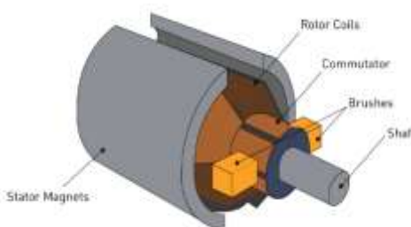
Figure1.4: DC Motor
