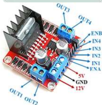
Figure1.6: Motor Driver
