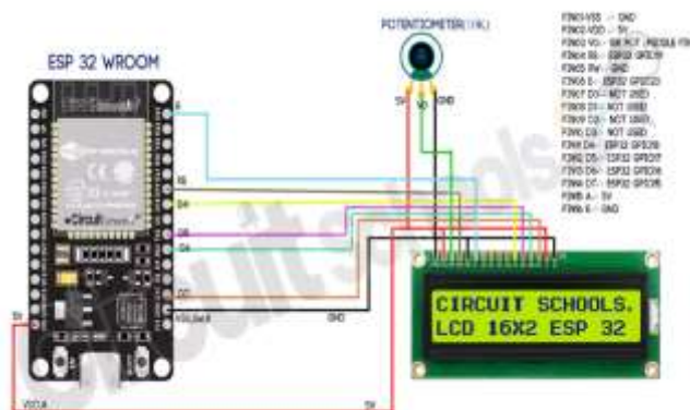
Figure1.7: LCD Display
