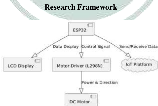
Figure1.3: Block Diagram
